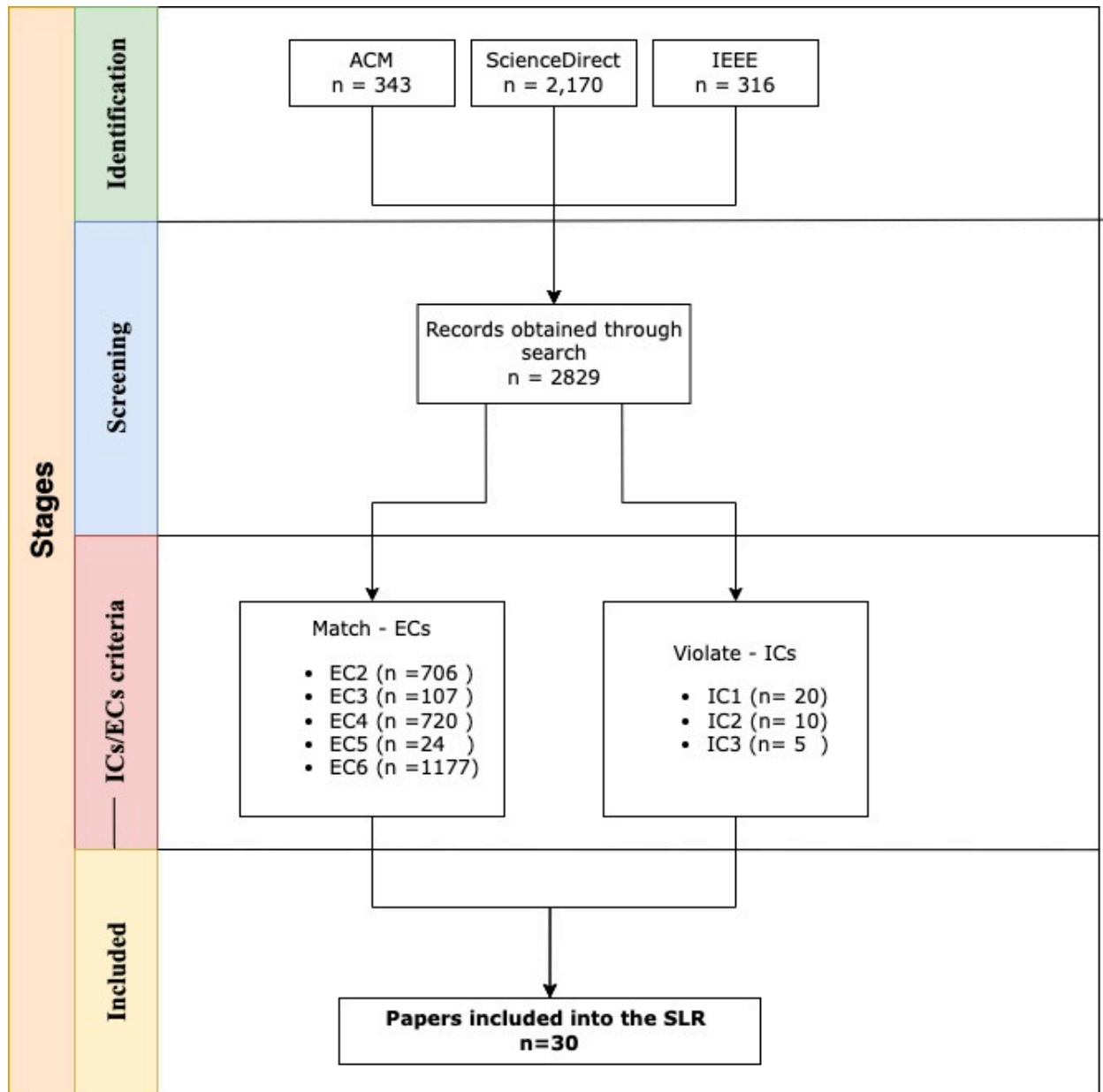
Figure 3.1: SLR diagram
